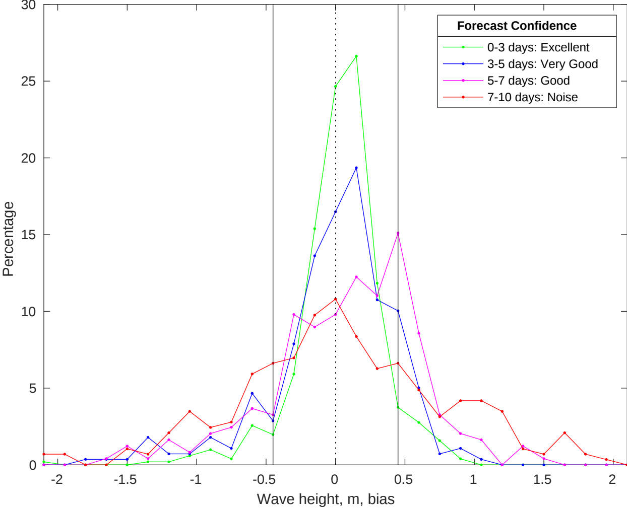
NDBC 46059 vs CMEMS Waves Bias Histogram: 03-Jan-2026
