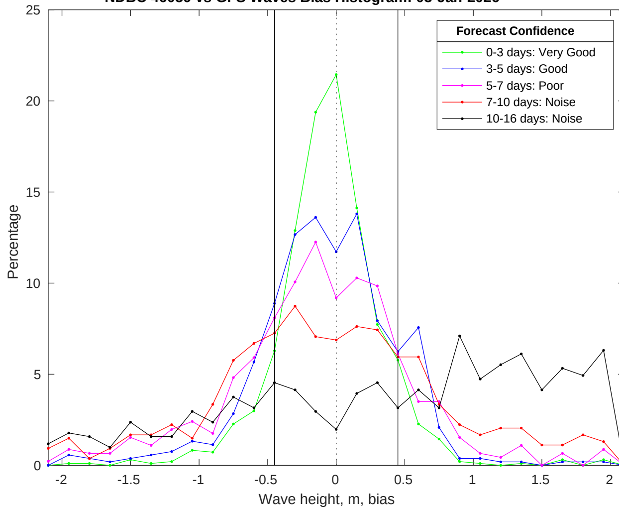
NDBC 46059 vs GFS Waves Bias Histogram: 03-Jan-2026
