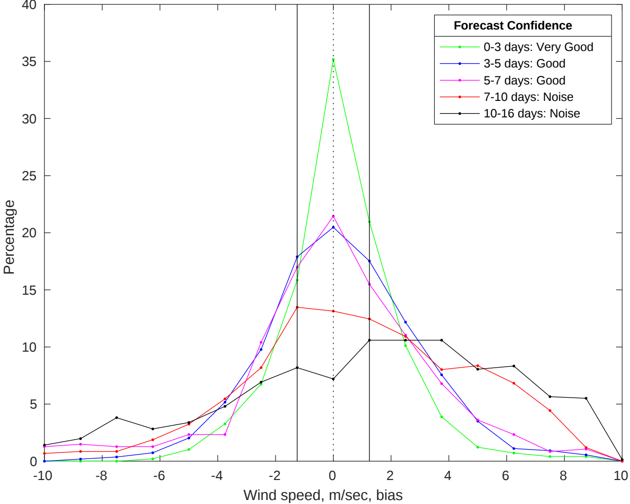
NDBC 46059 vs GFS Winds Bias Histogram: 03-Jan-2026
