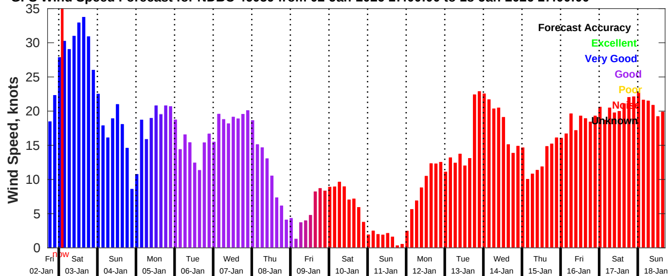
GFS Wind Speed Forecast for NDBC 46059 from 02-Jan-2026 17:00:00 to 18-Jan-2026 17:00:00
