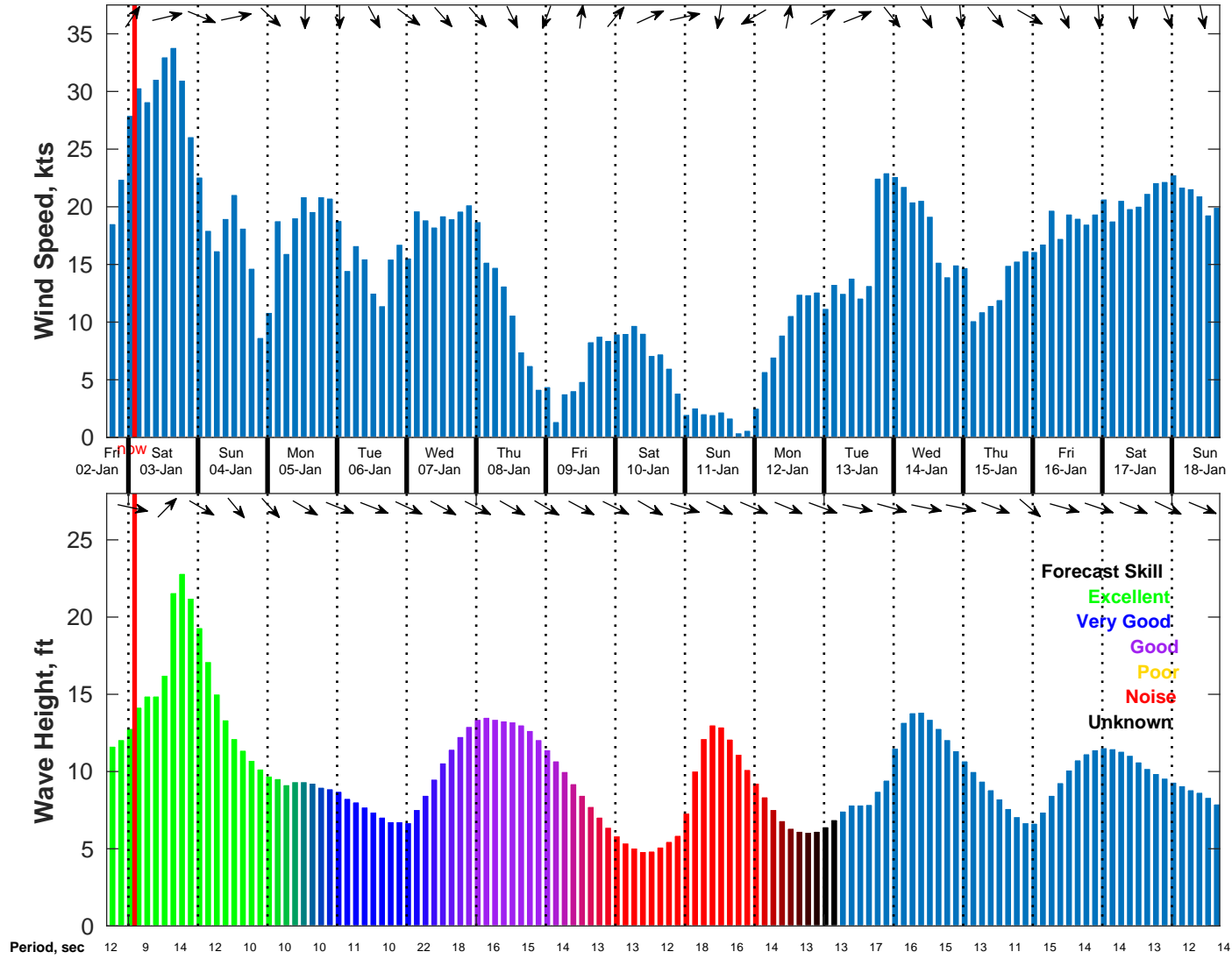
Wind & Wave Forecast for NDBC 46059 from 02-Jan-2026 17:00:00 to 18-Jan-2026 17:00:00
