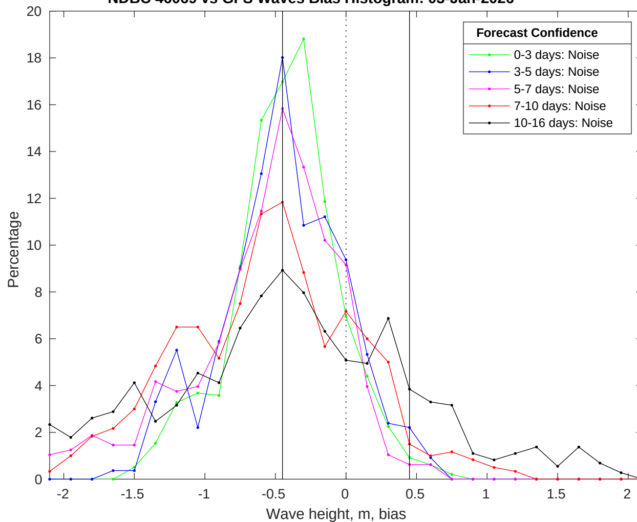
NDBC 46069 vs GFS Waves Bias Histogram: 03-Jan-2026
