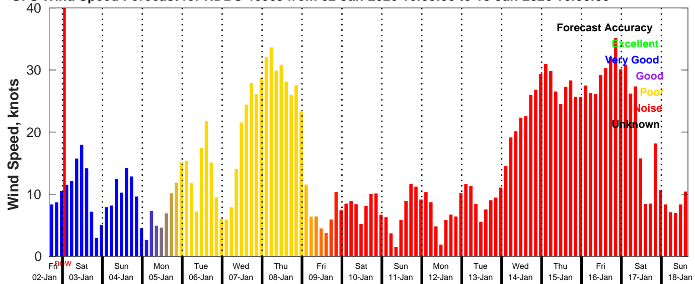
GFS Wind Speed Forecast for NDBC 46069 from 02-Jan-2026 16:00:00 to 18-Jan-2026 16:00:00
