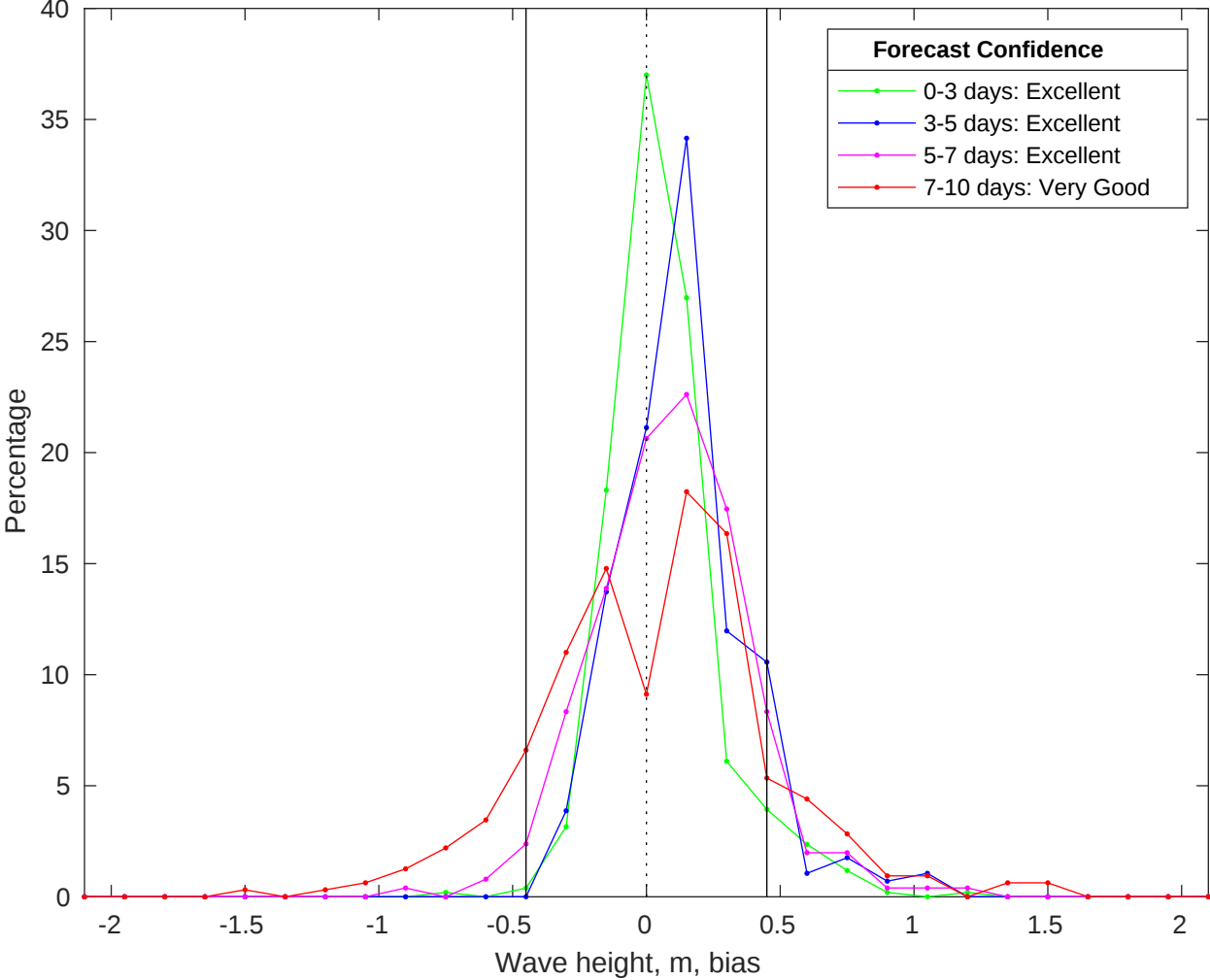
NDBC 46215 vs CMEMS Waves Bias Histogram: 03-Jan-2026
