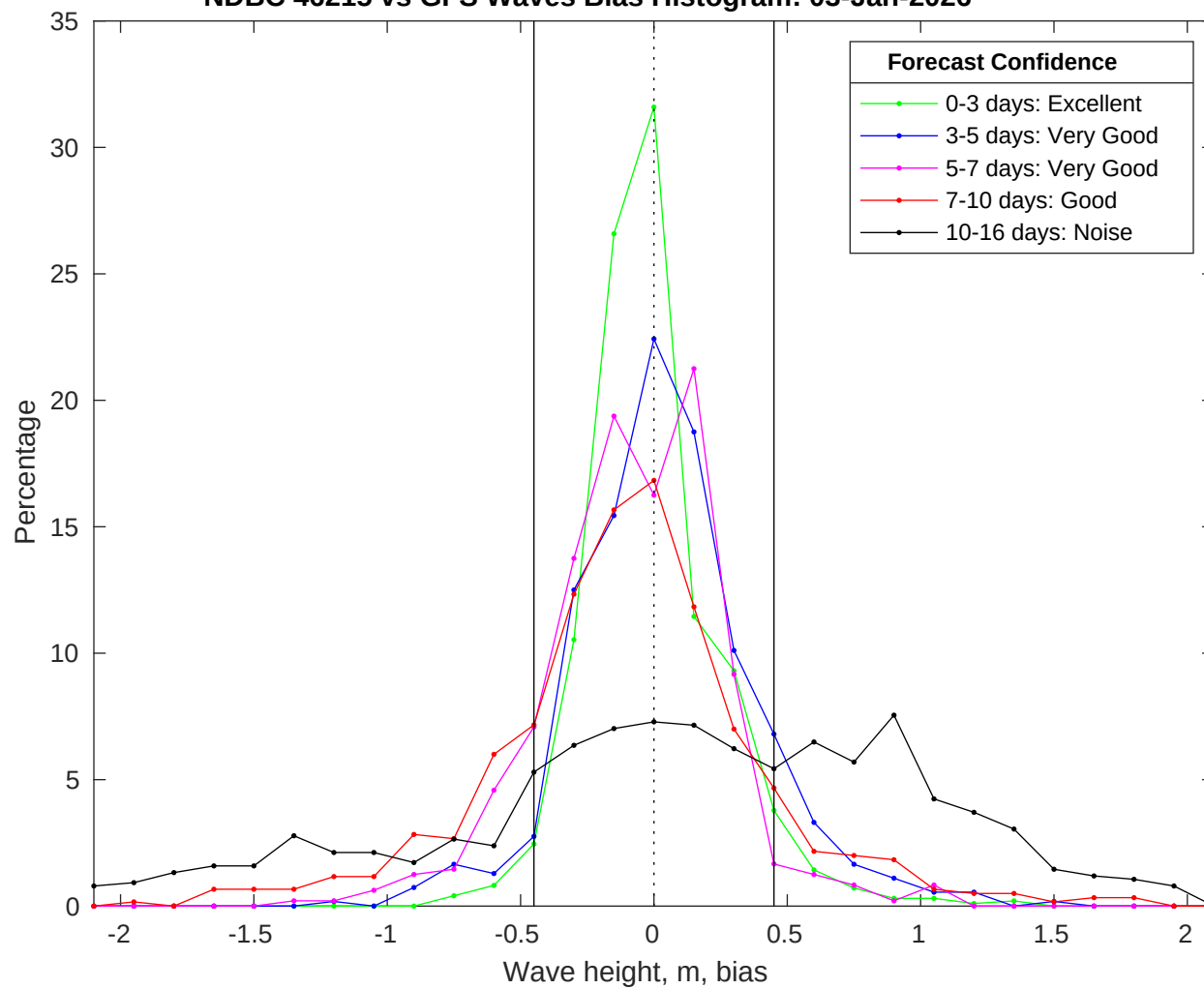
NDBC 46215 vs GFS Waves Bias Histogram: 03-Jan-2026
