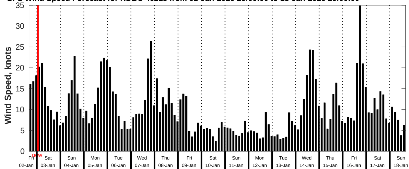
GFS Wind Speed Forecast for NDBC 46215 from 02-Jan-2026 16:00:00 to 18-Jan-2026 16:00:00
