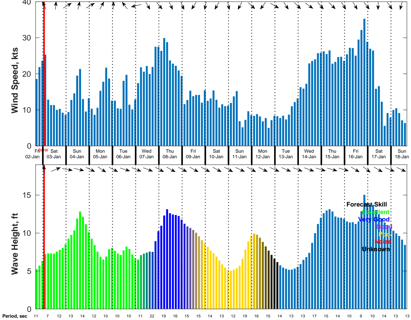
Wind & Wave Forecast for NDBC 46259 from 02-Jan-2026 16:00:00 to 18-Jan-2026 16:00:00
