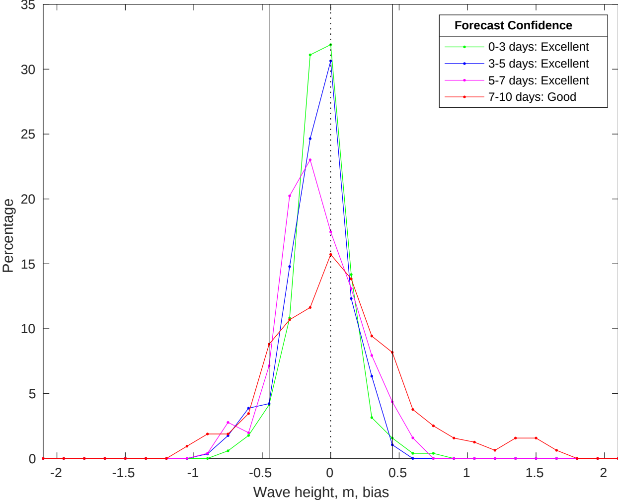
NDBC 51000 vs CMEMS Waves Bias Histogram: 03-Jan-2026
