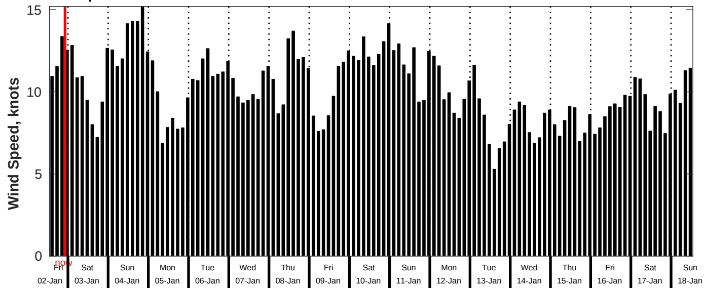
GFS Wind Speed Forecast for NDBC 51209 from 02-Jan-2026 13:00:00 to 18-Jan-2026 13:00:00
