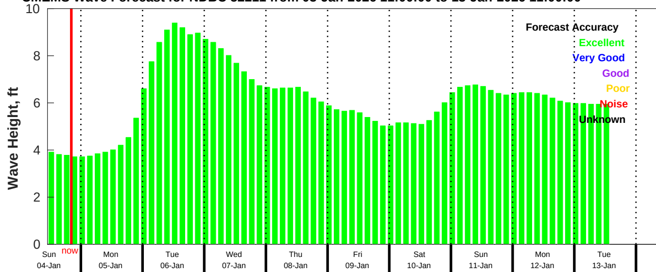
CMEMS Wave Forecast for NDBC 52211 from 03-Jan-2026 11:00:00 to 13-Jan-2026 11:00:00
