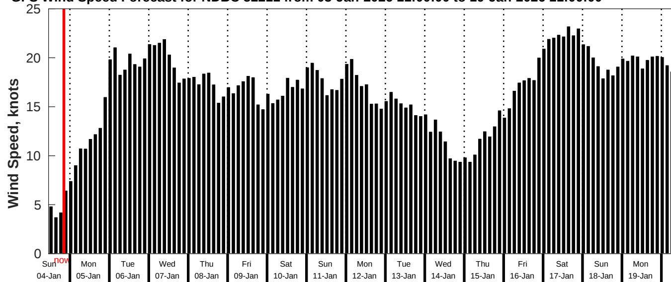
GFS Wind Speed Forecast for NDBC 52211 from 03-Jan-2026 11:00:00 to 19-Jan-2026 11:00:00
