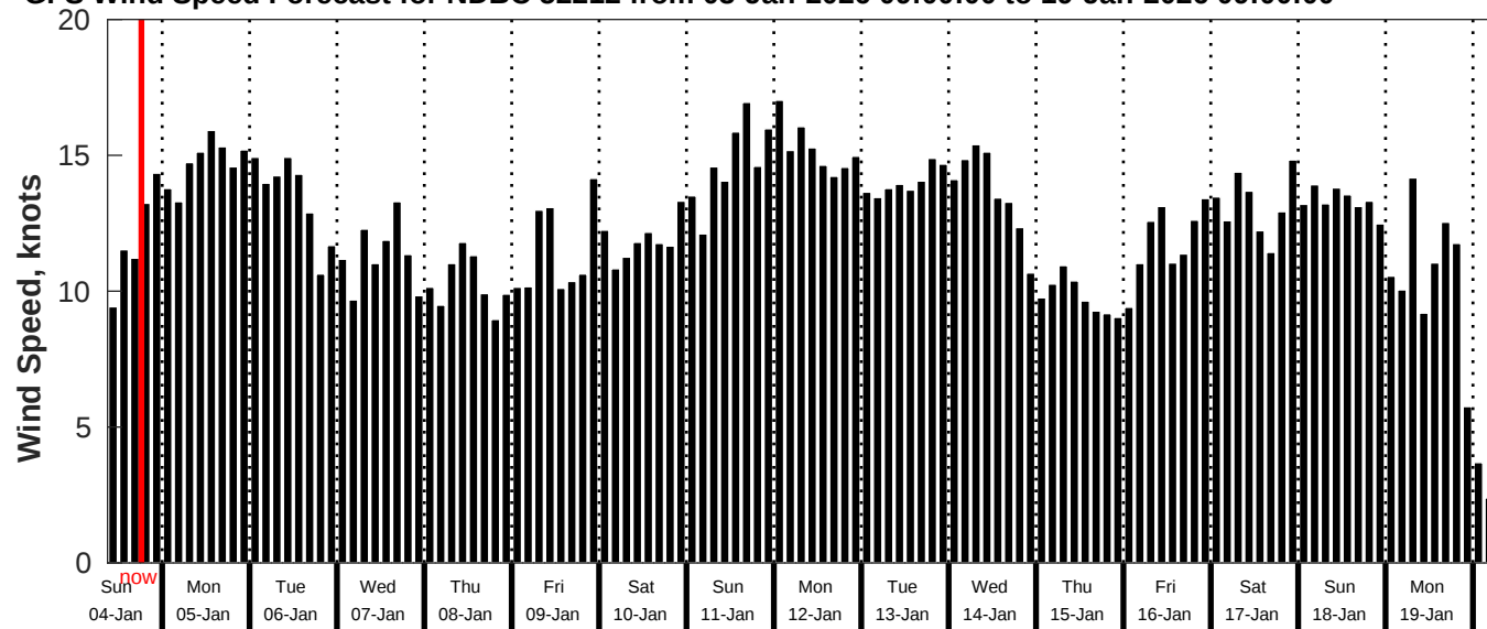
GFS Wind Speed Forecast for NDBC 52212 from 03-Jan-2026 09:00:00 to 19-Jan-2026 09:00:00
