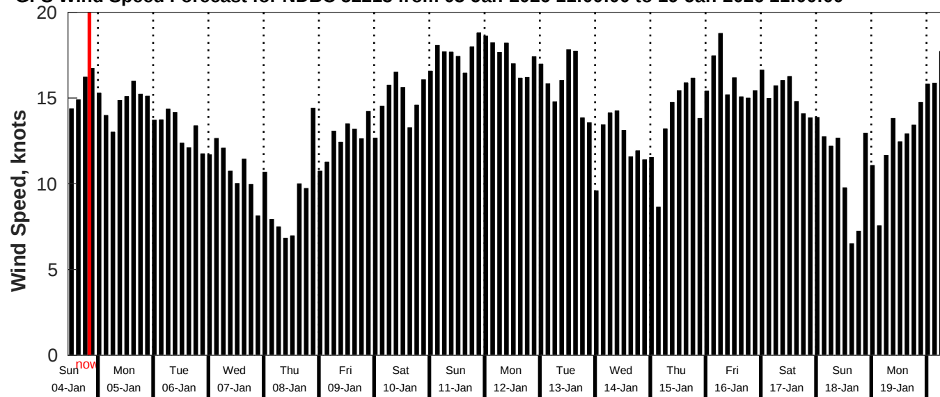
GFS Wind Speed Forecast for NDBC 52213 from 03-Jan-2026 11:00:00 to 19-Jan-2026 11:00:00
