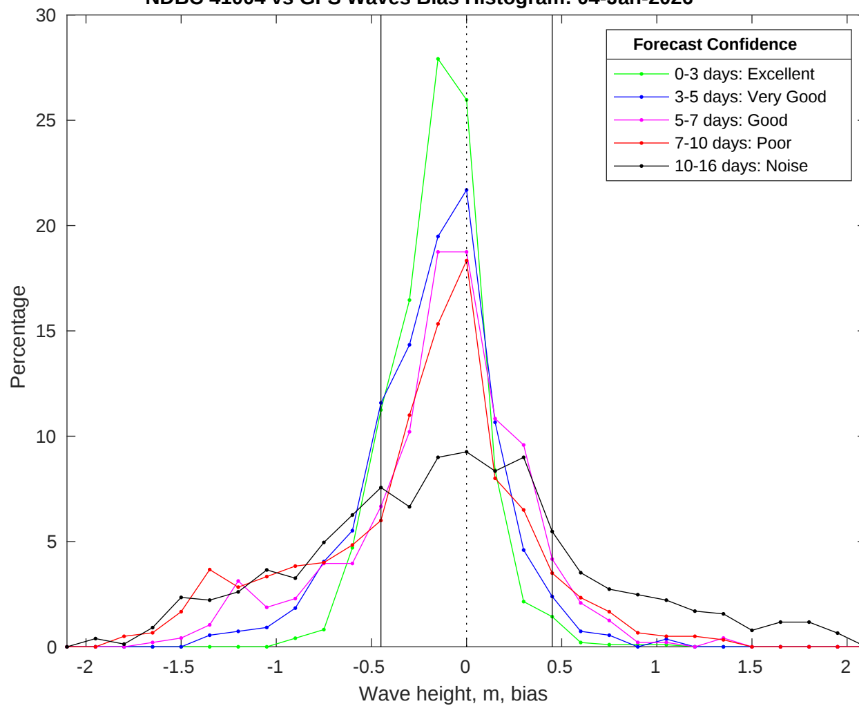
NDBC 41004 vs GFS Waves Bias Histogram: 04-Jan-2026
