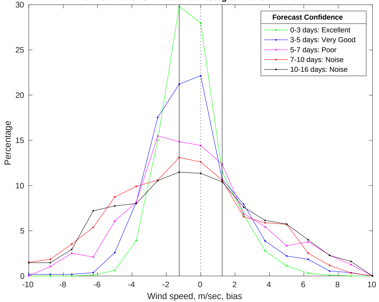
NDBC 41004 vs GFS Winds Bias Histogram: 04-Jan-2026
