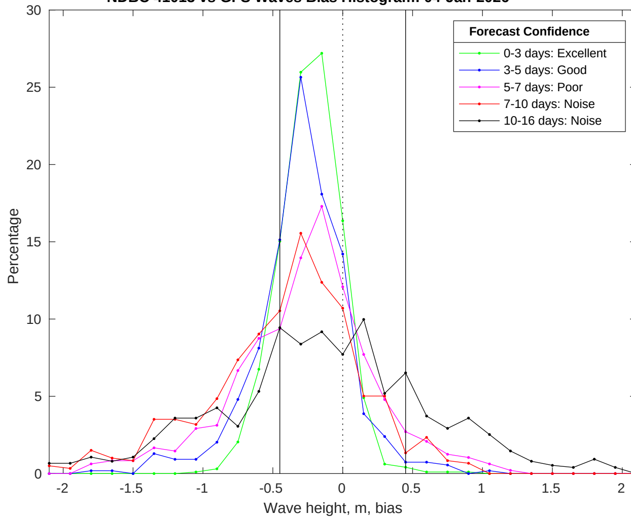
NDBC 41013 vs GFS Waves Bias Histogram: 04-Jan-2026
