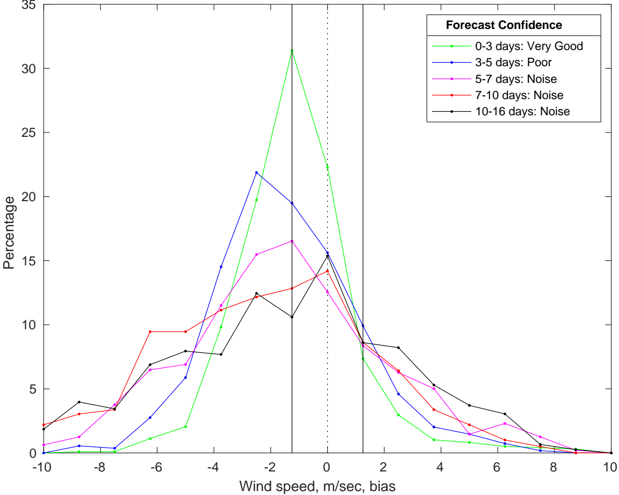
NDBC 41013 vs GFS Winds Bias Histogram: 04-Jan-2026
