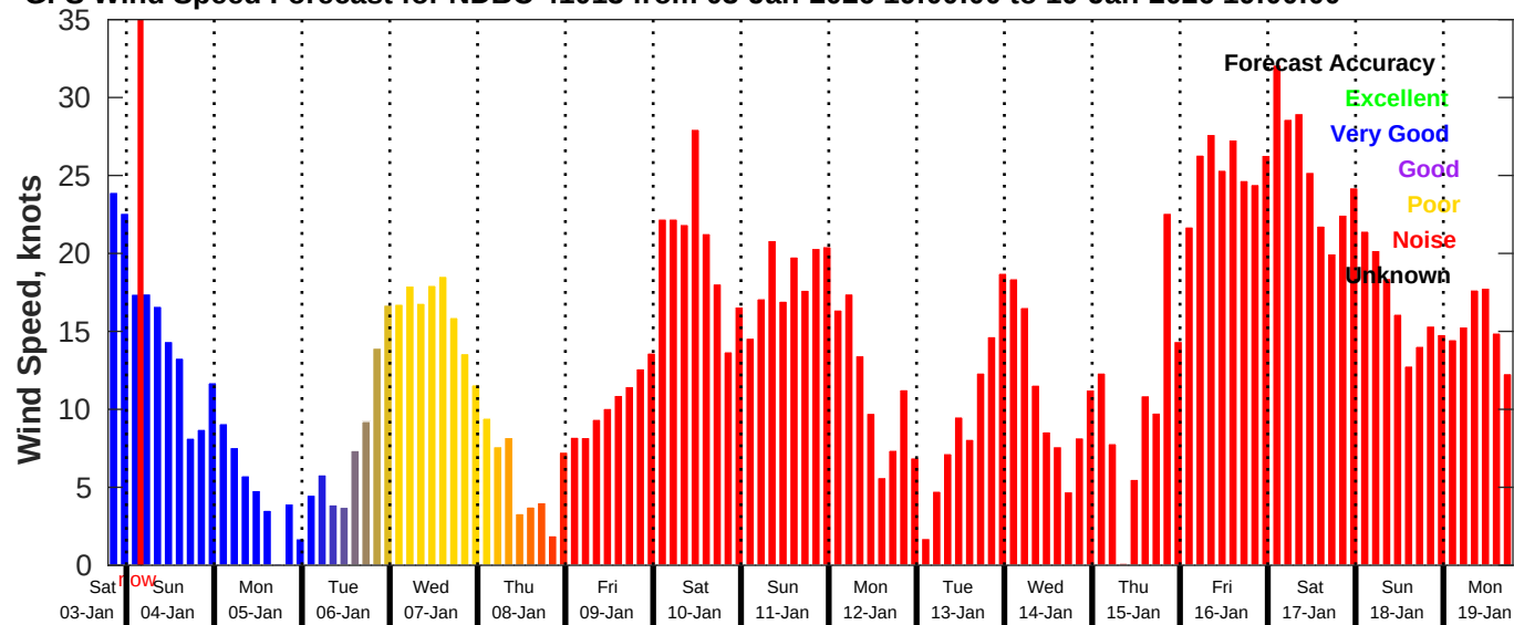
GFS Wind Speed Forecast for NDBC 41013 from 03-Jan-2026 19:00:00 to 19-Jan-2026 19:00:00
