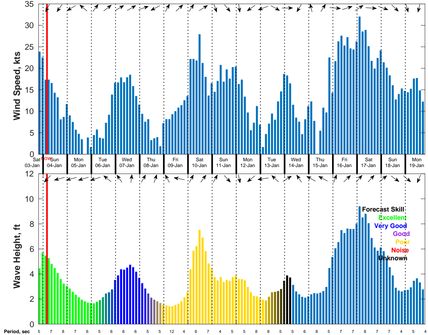
Wind & Wave Forecast for NDBC 41013 from 03-Jan-2026 19:00:00 to 19-Jan-2026 19:00:00
