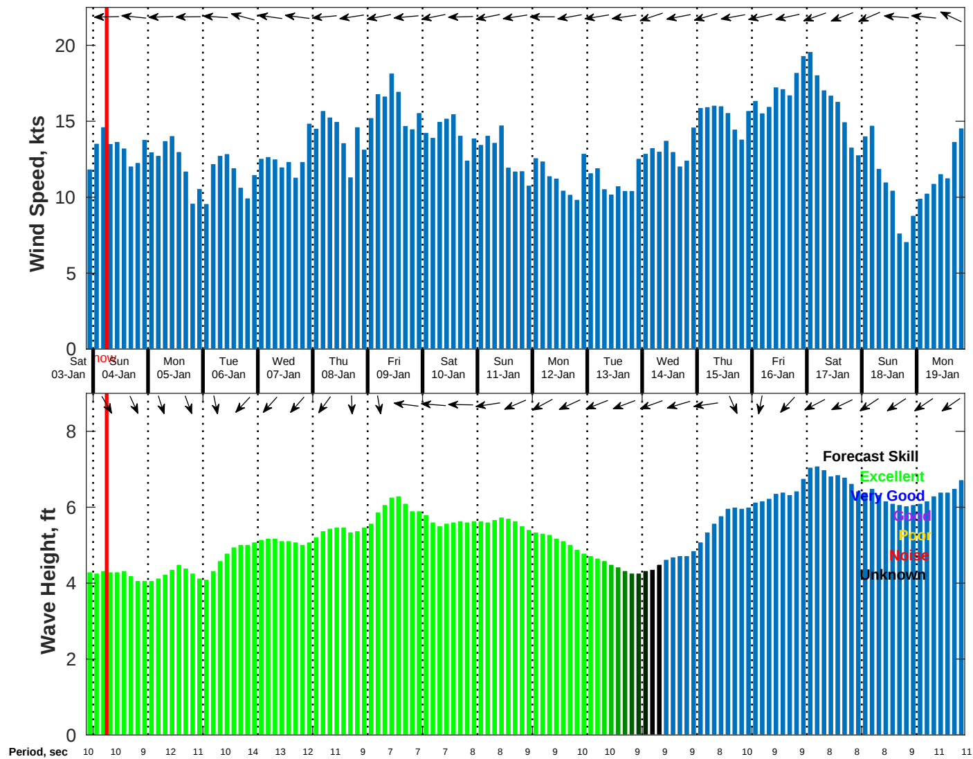
Wind & Wave Forecast for NDBC 41040 from 03-Jan-2026 21:00:00 to 19-Jan-2026 21:00:00
