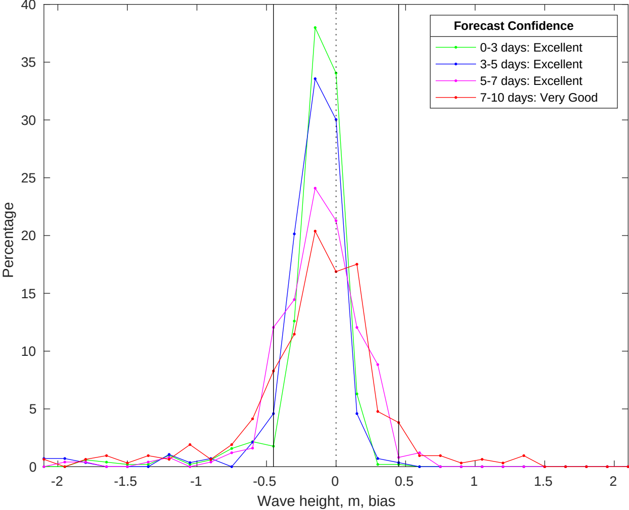
NDBC 42019 vs CMEMS Waves Bias Histogram: 04-Jan-2026
