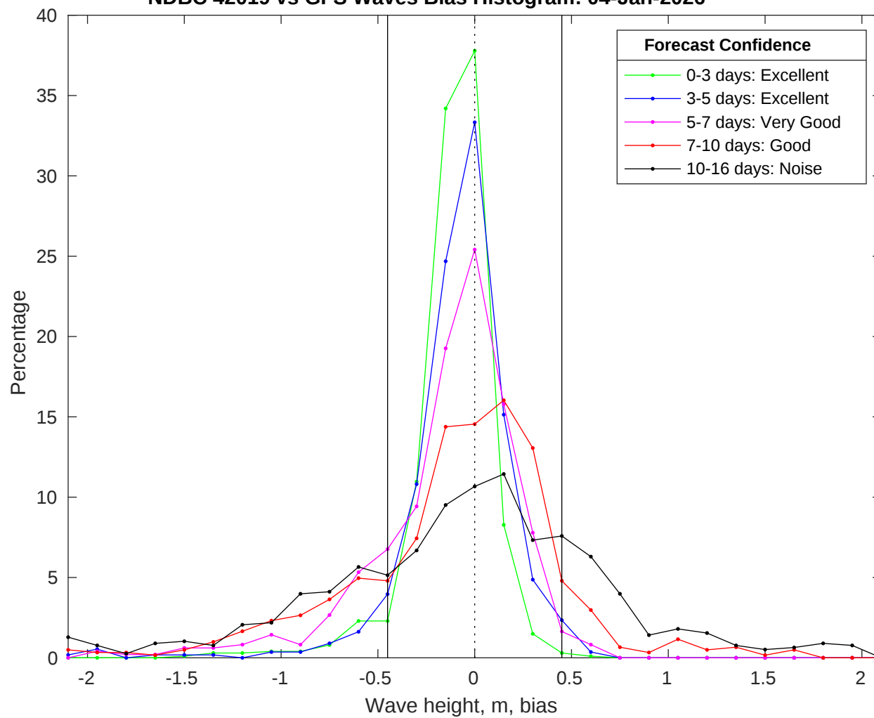
NDBC 42019 vs GFS Waves Bias Histogram: 04-Jan-2026
