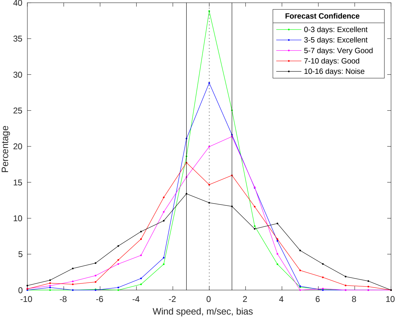
NDBC 42019 vs GFS Winds Bias Histogram: 04-Jan-2026
