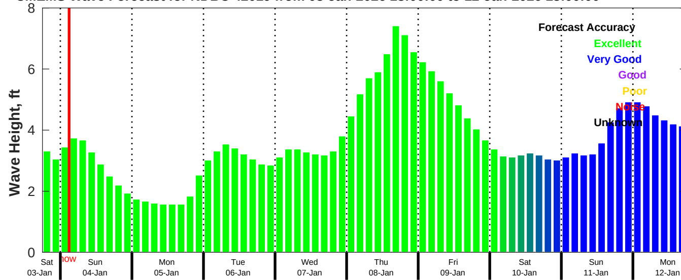
CMEMS Wave Forecast for NDBC 42019 from 03-Jan-2026 18:00:00 to 12-Jan-2026 18:00:00
