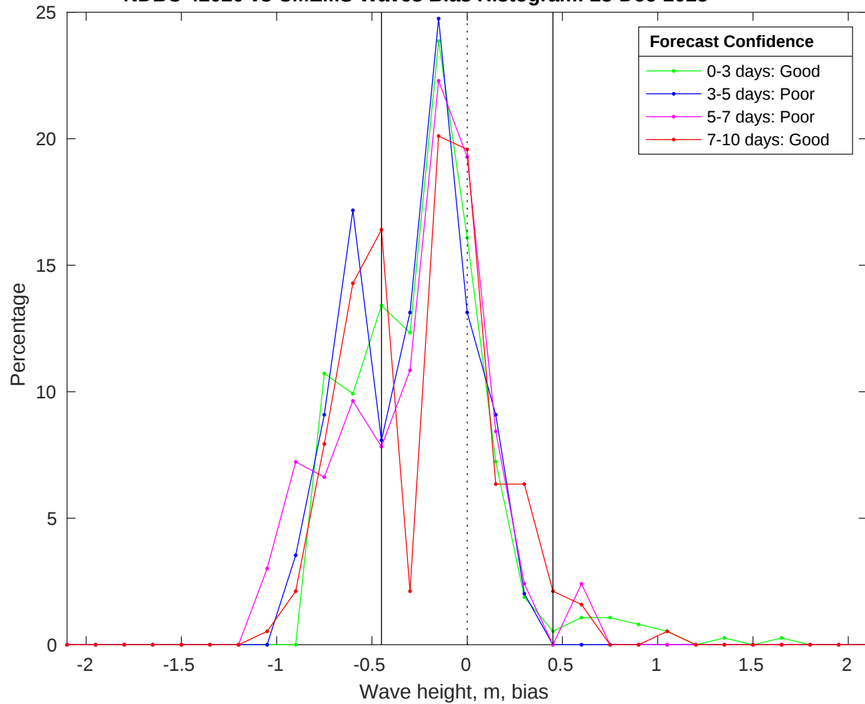
NDBC 42020 vs CMEMS Waves Bias Histogram: 28-Dec-2025
