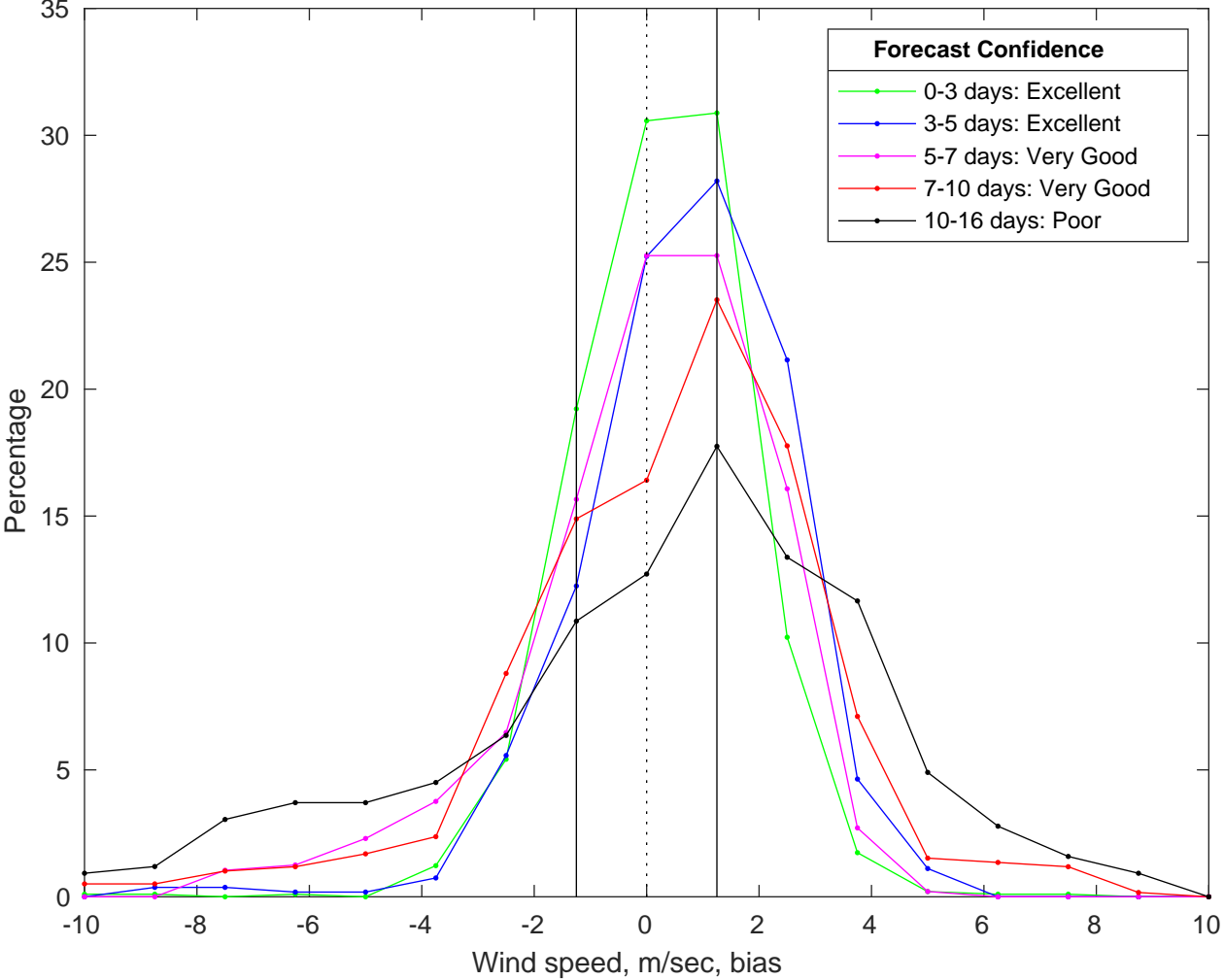
NDBC 42020 vs GFS Winds Bias Histogram: 02-Jan-2026
