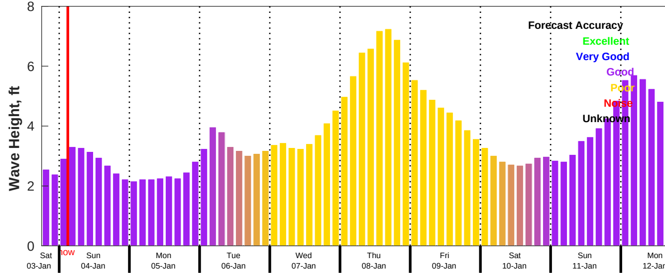
CMEMS Wave Forecast for NDBC 42020 from 03-Jan-2026 18:00:00 to 12-Jan-2026 18:00:00
