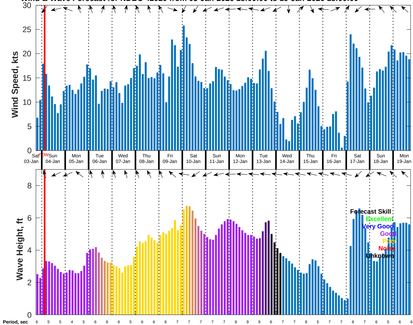
Wind & Wave Forecast for NDBC 42020 from 03-Jan-2026 18:00:00 to 19-Jan-2026 18:00:00
