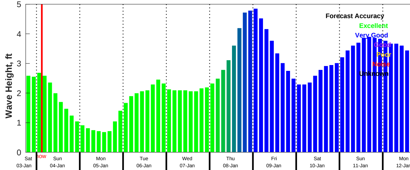
CMEMS Wave Forecast for NDBC 42035 from 03-Jan-2026 18:00:00 to 12-Jan-2026 18:00:00
