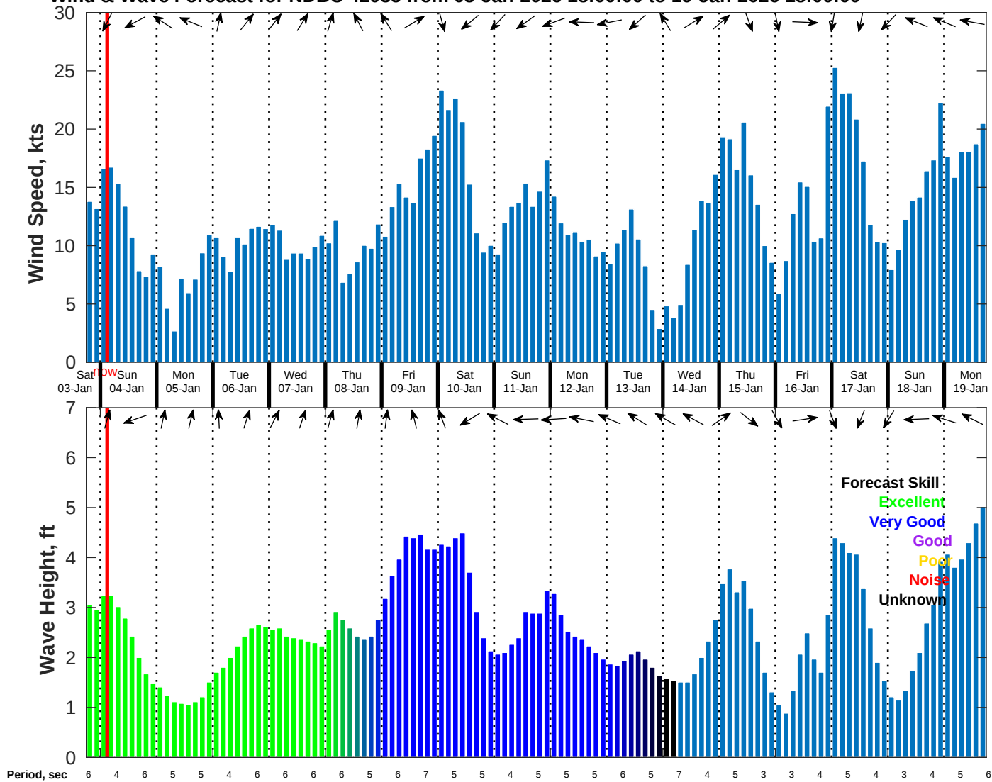
Wind & Wave Forecast for NDBC 42035 from 03-Jan-2026 18:00:00 to 19-Jan-2026 18:00:00
