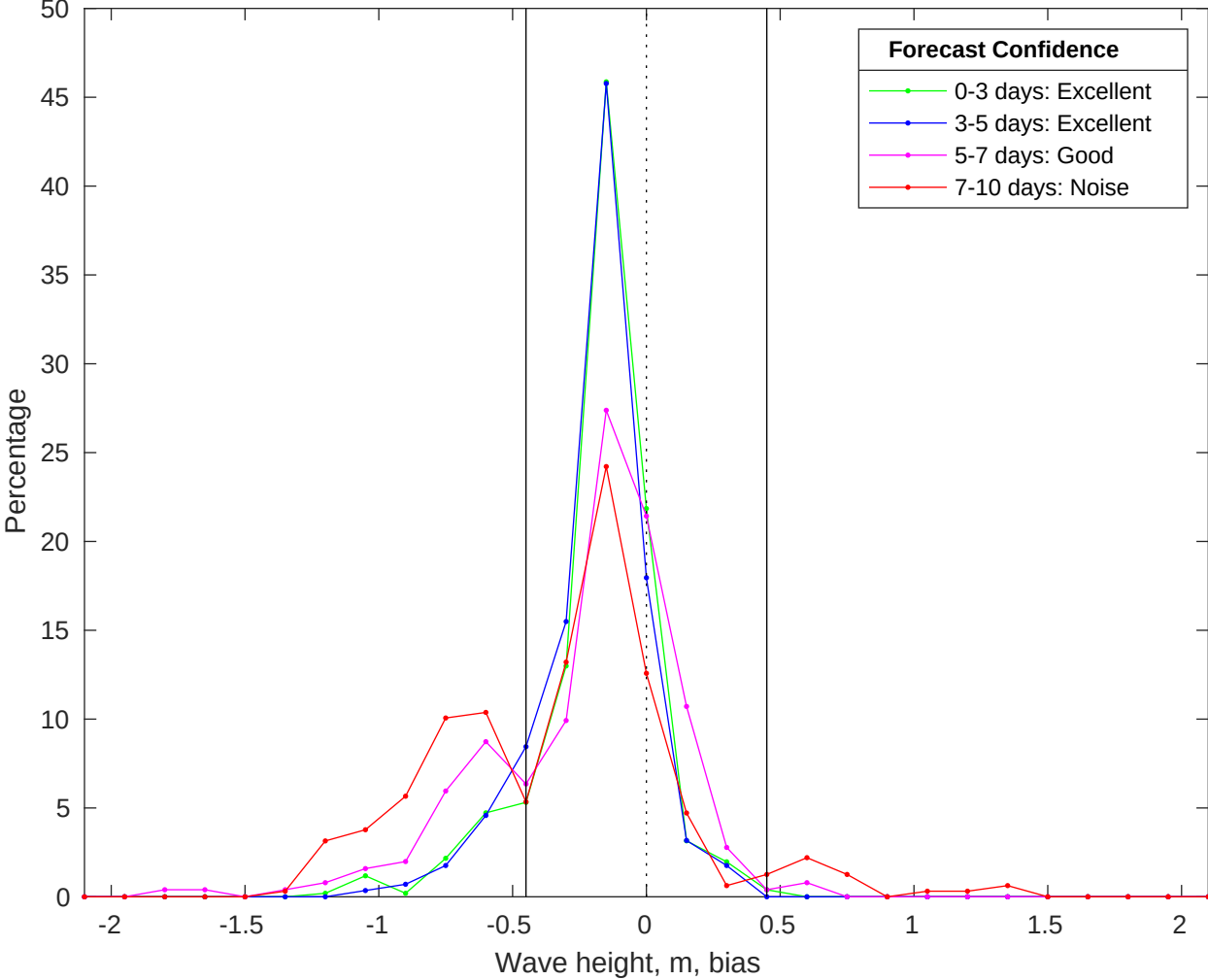
NDBC 42036 vs CMEMS Waves Bias Histogram: 04-Jan-2026
