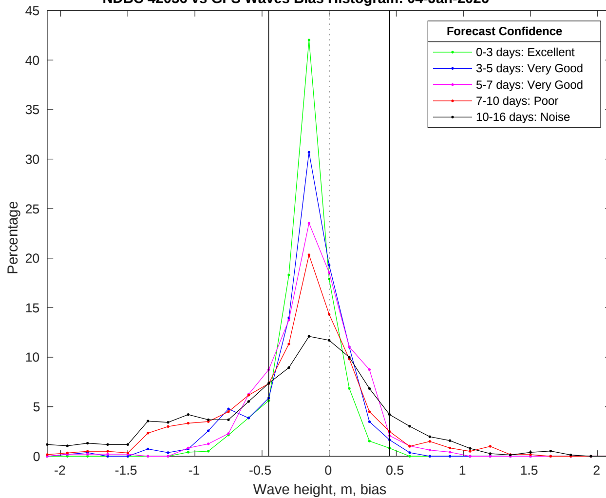
NDBC 42036 vs GFS Waves Bias Histogram: 04-Jan-2026
