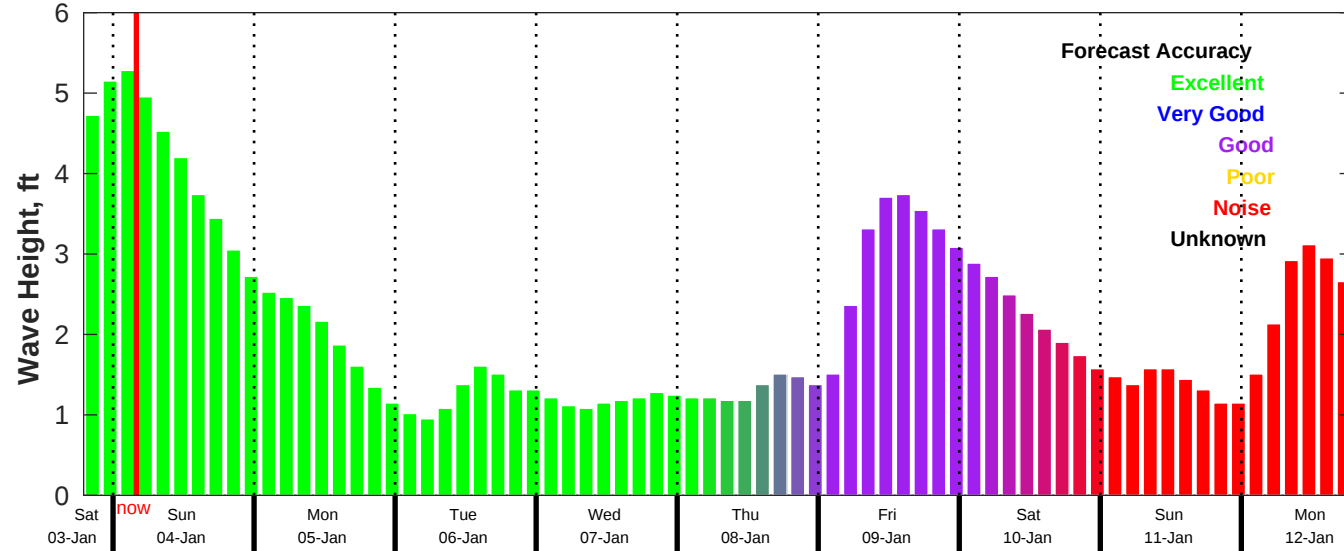
CMEMS Wave Forecast for NDBC 42036 from 03-Jan-2026 19:00:00 to 12-Jan-2026 19:00:00
