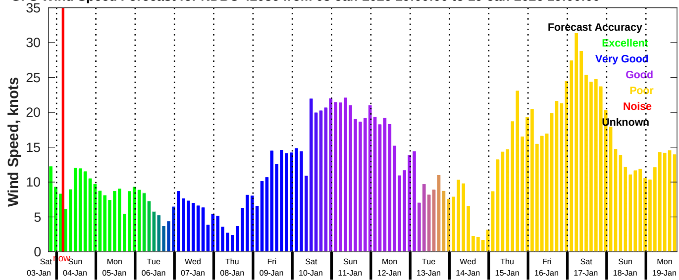
GFS Wind Speed Forecast for NDBC 42036 from 03-Jan-2026 19:00:00 to 19-Jan-2026 19:00:00
