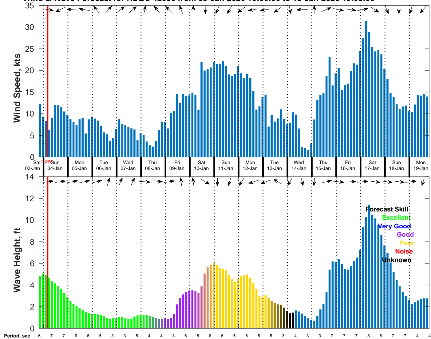
Wind & Wave Forecast for NDBC 42036 from 03-Jan-2026 19:00:00 to 19-Jan-2026 19:00:00
