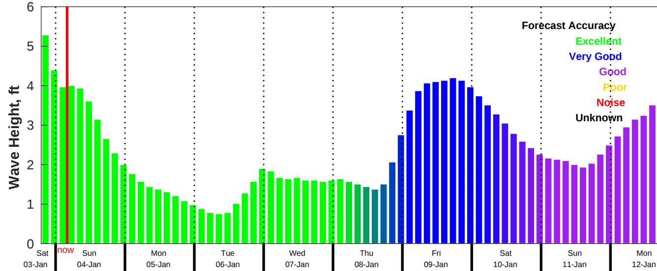
CMEMS Wave Forecast for NDBC 42040 from 03-Jan-2026 19:00:00 to 12-Jan-2026 19:00:00
