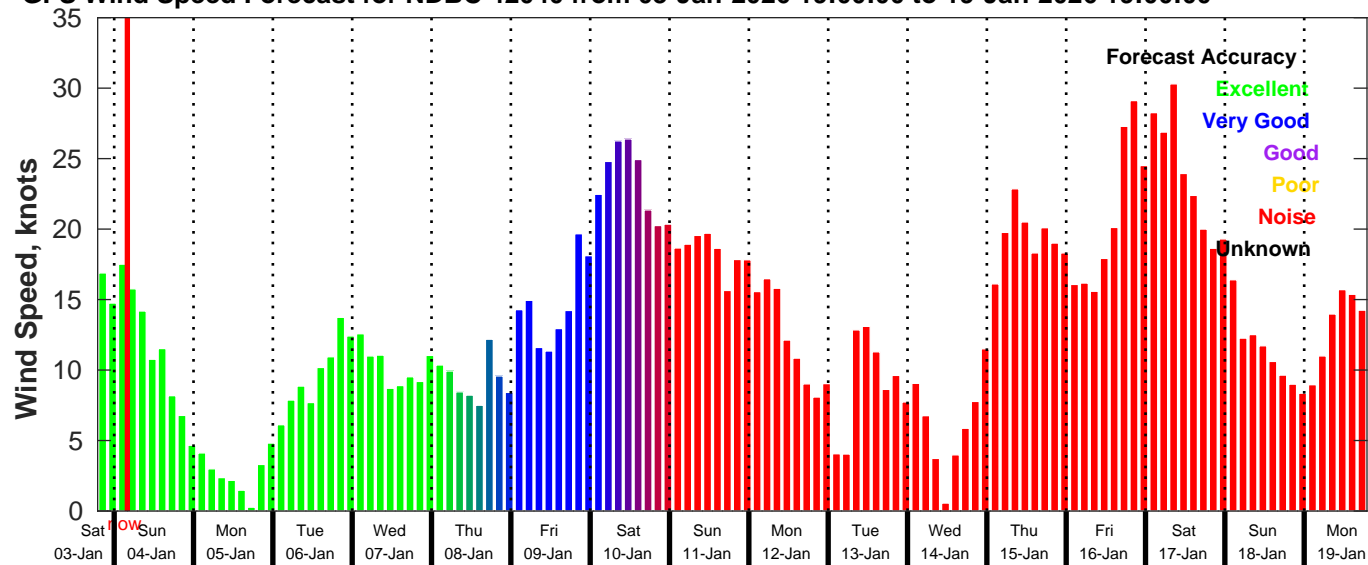
GFS Wind Speed Forecast for NDBC 42040 from 03-Jan-2026 19:00:00 to 19-Jan-2026 19:00:00
