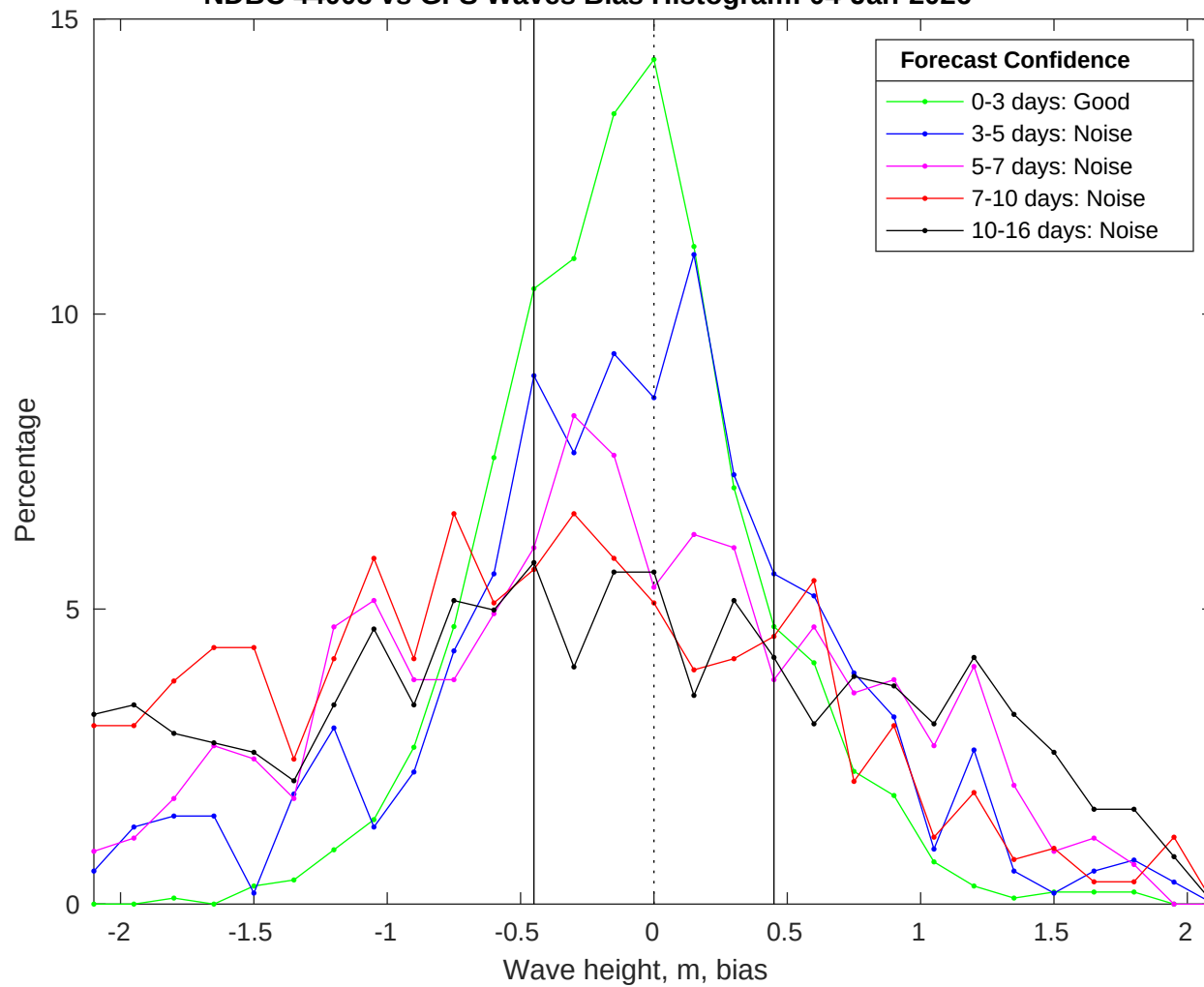
NDBC 44008 vs GFS Waves Bias Histogram: 04-Jan-2026
