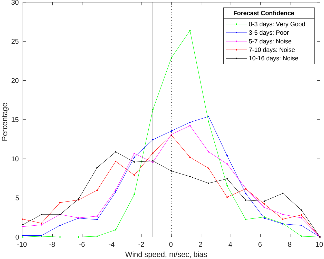
NDBC 44008 vs GFS Winds Bias Histogram: 04-Jan-2026
