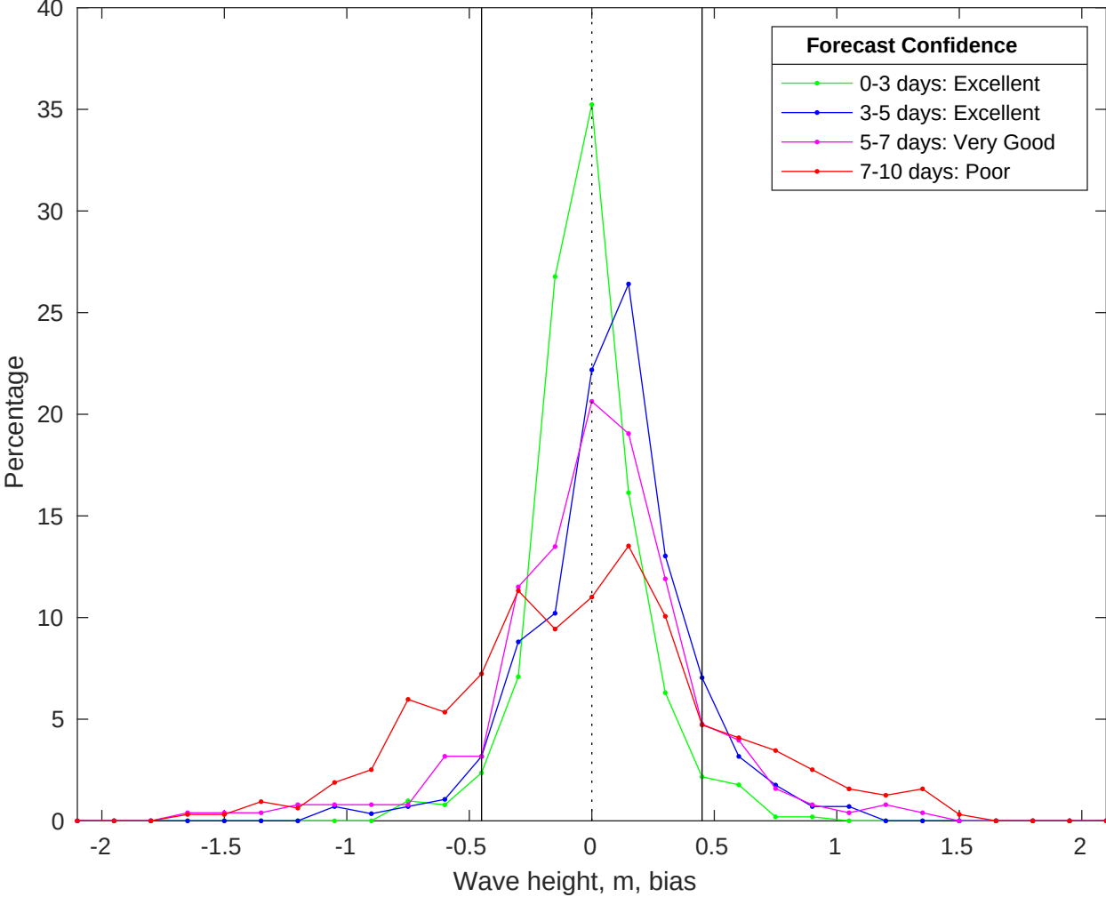
NDBC 46011 vs CMEMS Waves Bias Histogram: 04-Jan-2026
