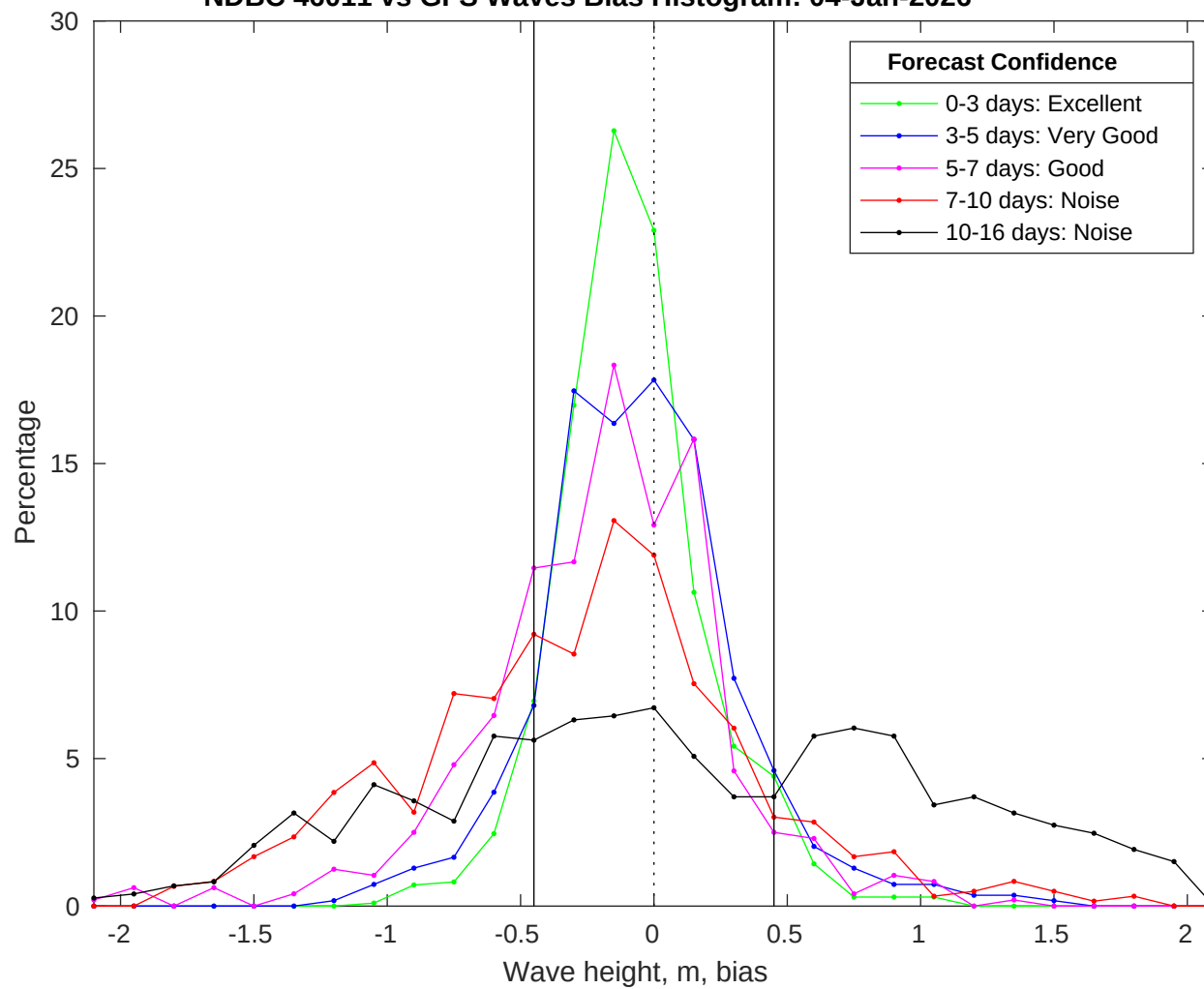
NDBC 46011 vs GFS Waves Bias Histogram: 04-Jan-2026
