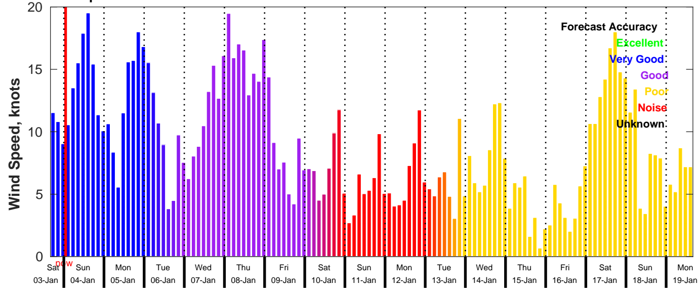
GFS Wind Speed Forecast for NDBC 46011 from 03-Jan-2026 16:00:00 to 19-Jan-2026 16:00:00
