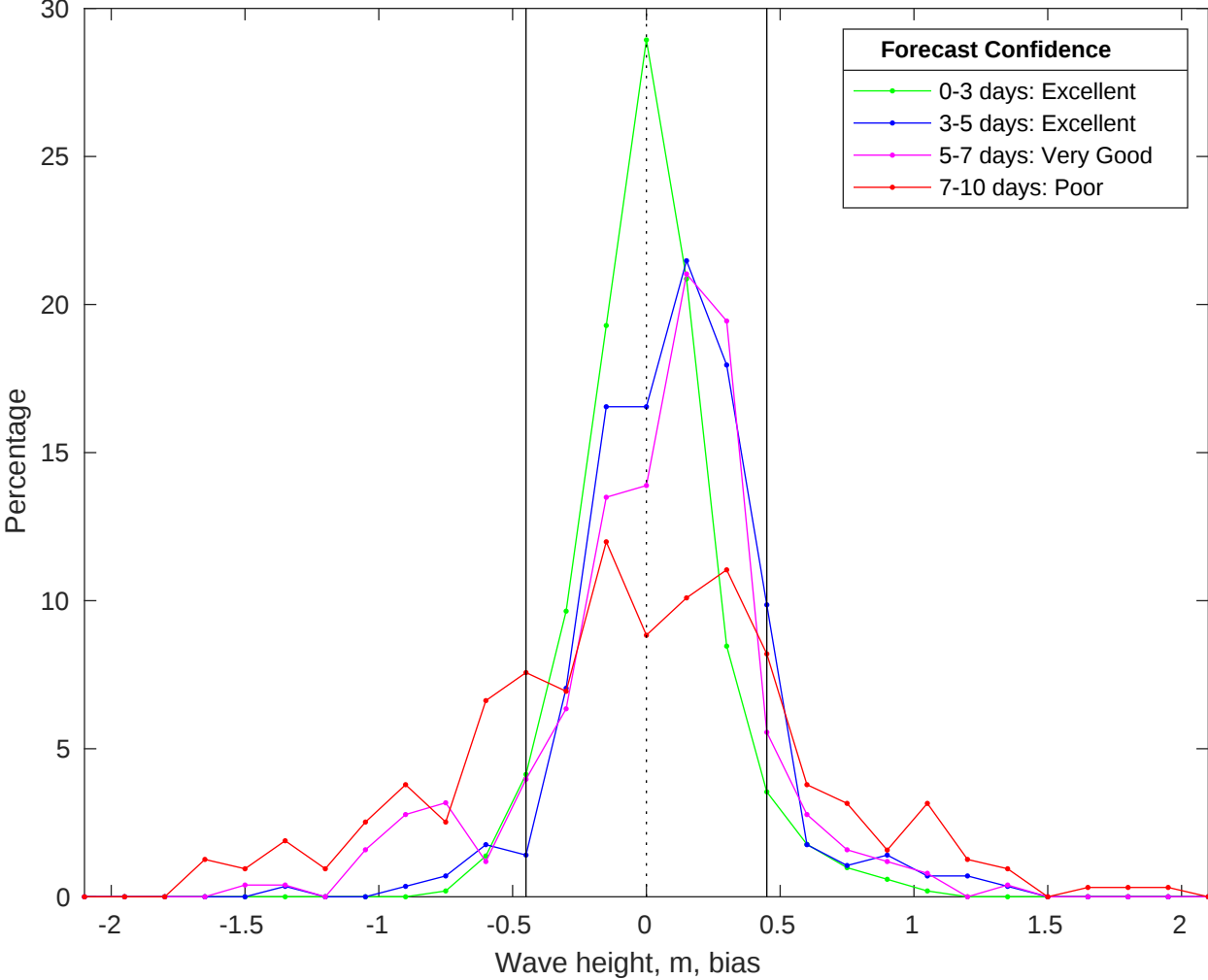
NDBC 46028 vs CMEMS Waves Bias Histogram: 04-Jan-2026
