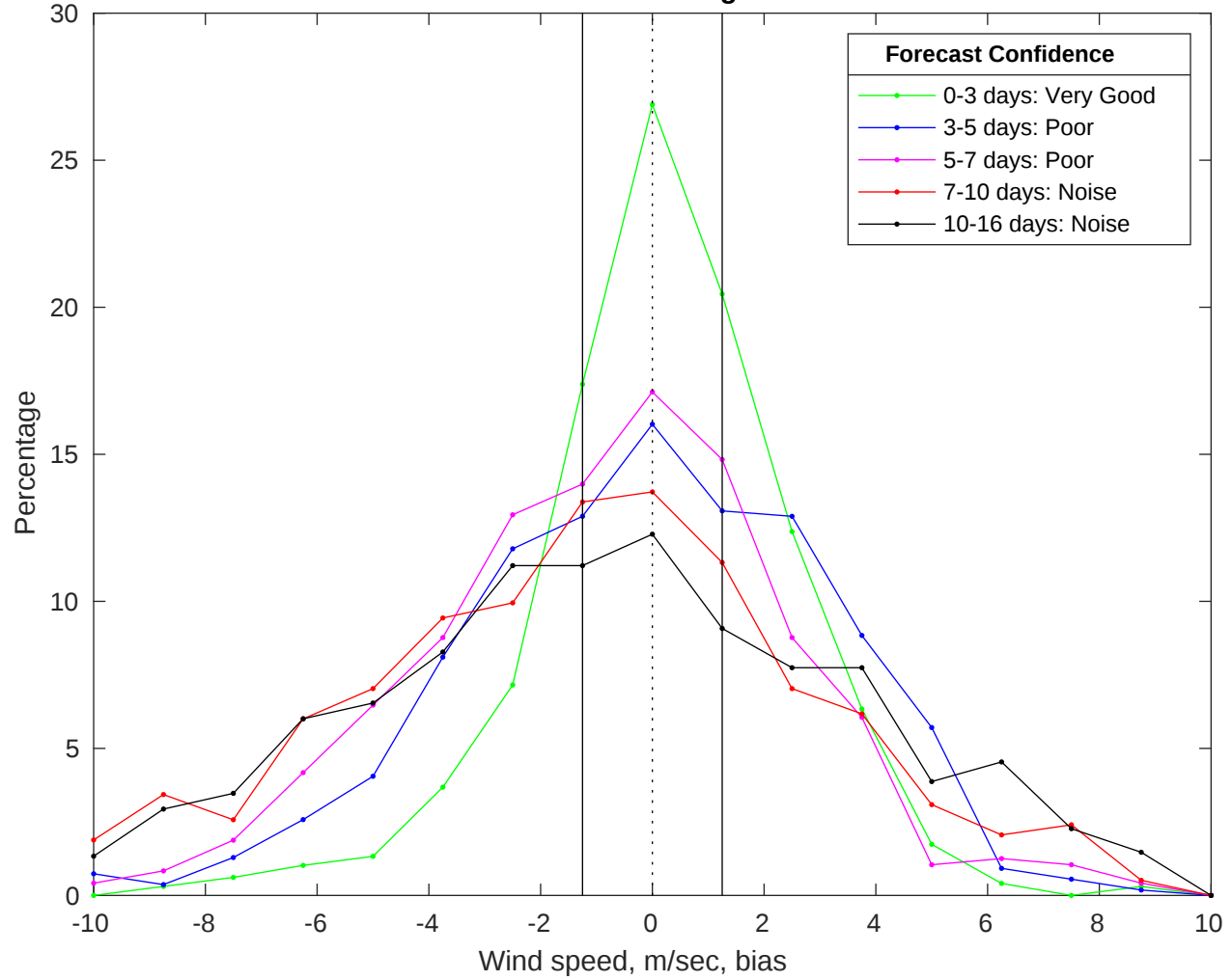
NDBC 46028 vs GFS Winds Bias Histogram: 04-Jan-2026
