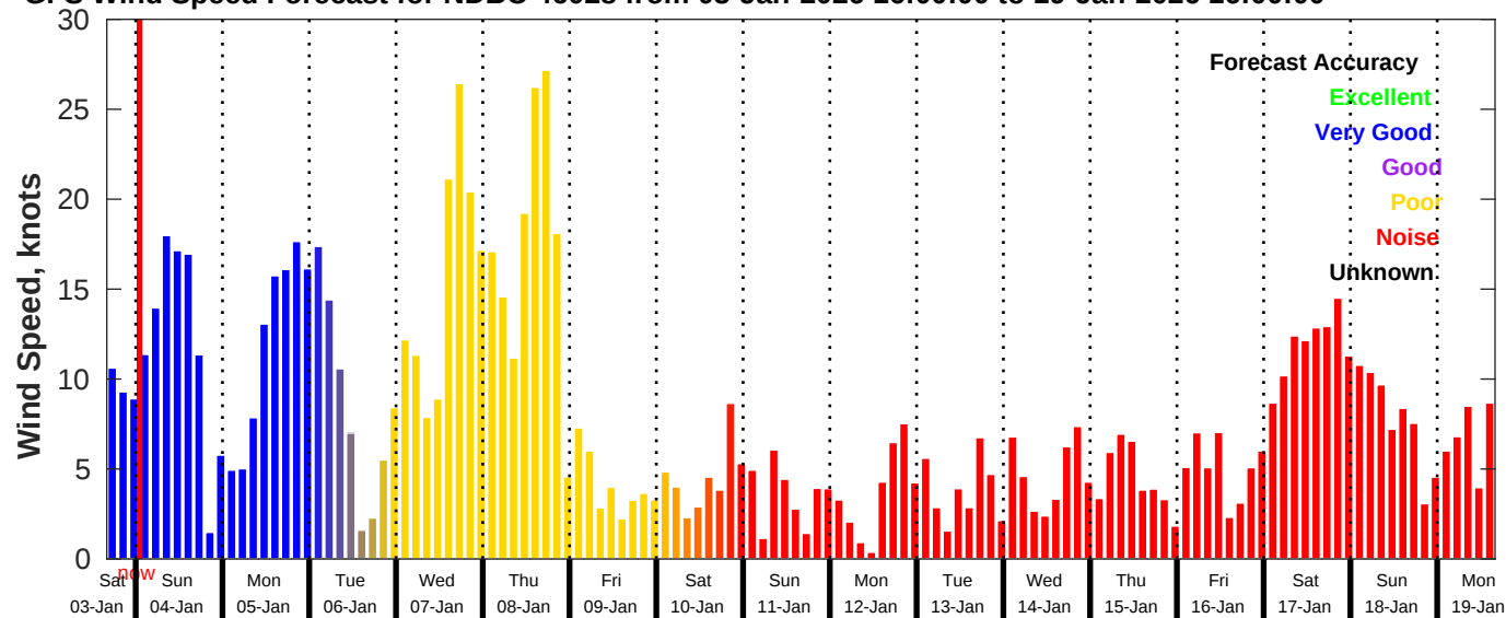
GFS Wind Speed Forecast for NDBC 46028 from 03-Jan-2026 16:00:00 to 19-Jan-2026 16:00:00
