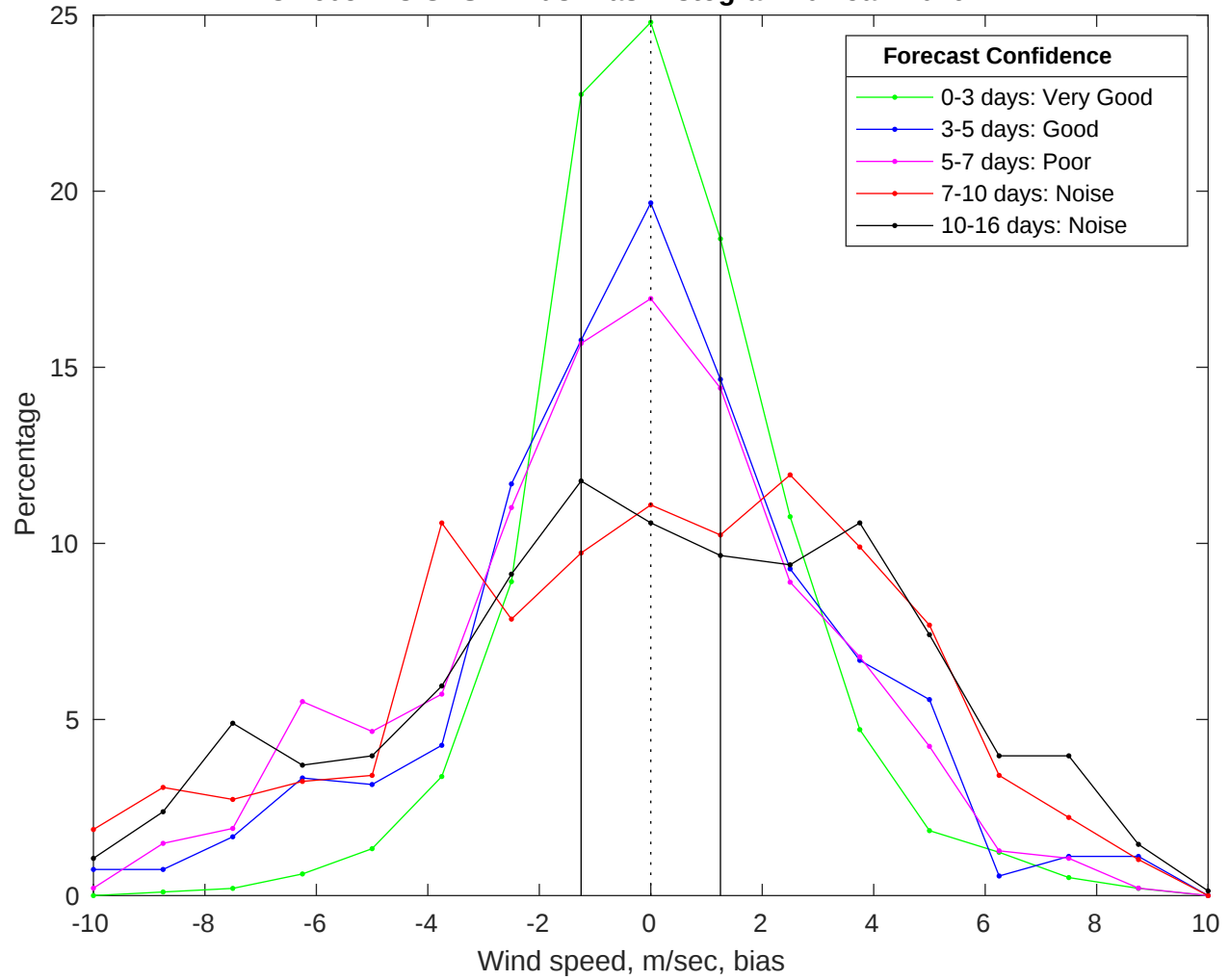
NDBC 46054 vs GFS Winds Bias Histogram: 04-Jan-2026
